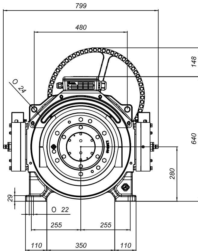
MGX80 GEARLESS MACHINE Ø400mm TRACTION SHEAVE 4 ROPES Ø10mm p.17mm
